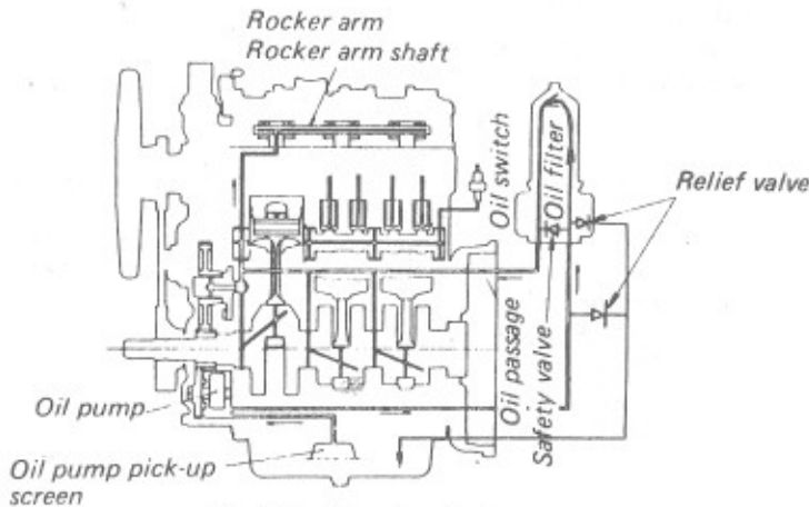
Fig. 8. Lubrication System
