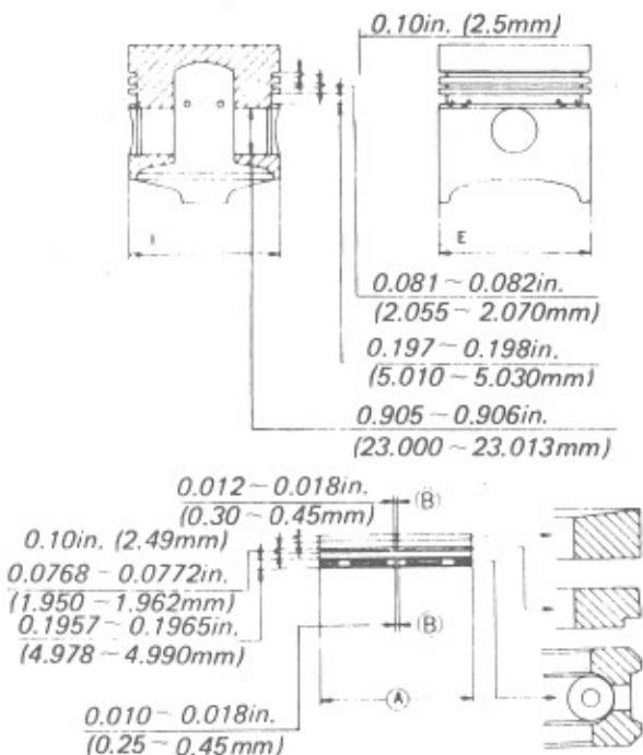
Fig. 26. Standard Dimensions of Piston and Piston Rings
