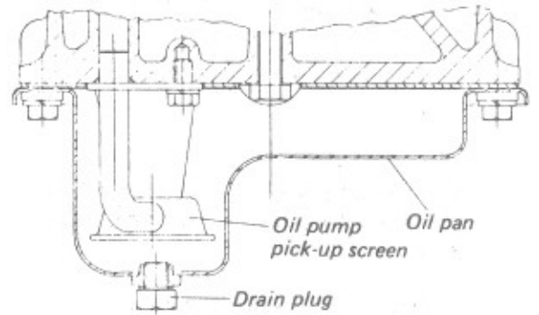
Fig. 9. Detail of Oil Pump Pick-up
