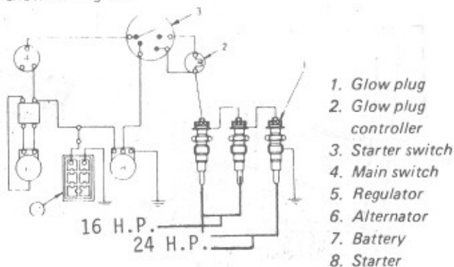
Fig. 44. Circuit Diagram for Glow Plugs
