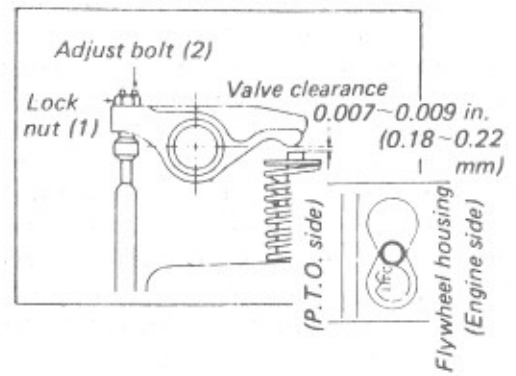
Fig. 17. Adjustment of Valve Clearance
