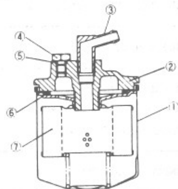
Fig. 2. Fuel Filter
